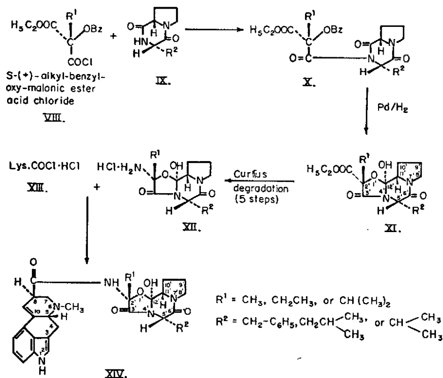
Fig. 5 Synthesis of peptide-type ergot alkaloids.
