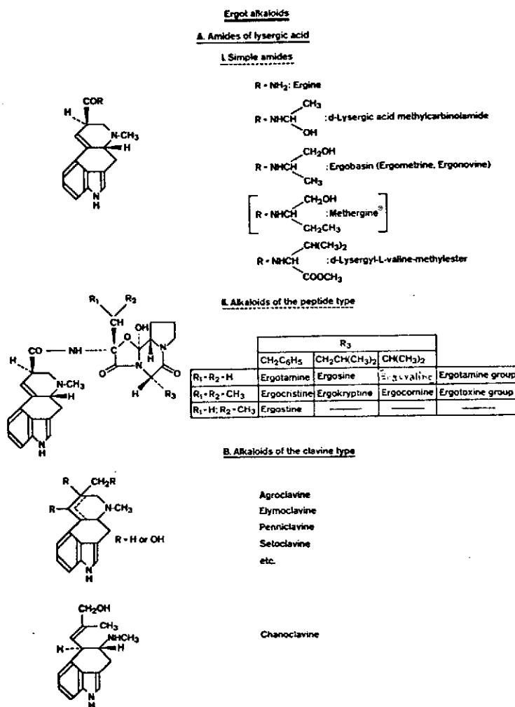
Fig. 3 Ergot alkaloids.
