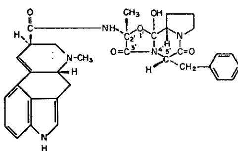
XX Ergotamine
