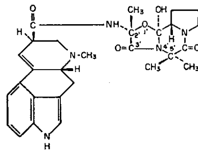
XXI 5'-Methylergoalanine
